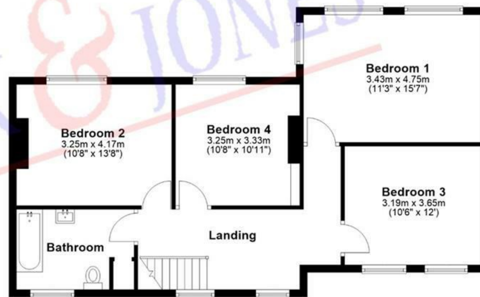
First Floor
